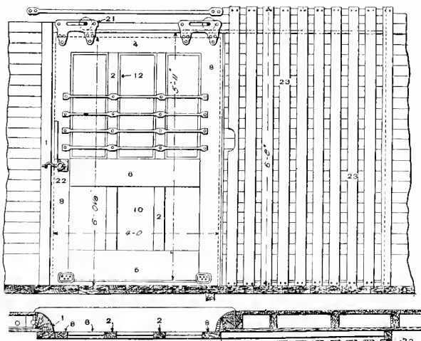
Fig. 1792. BAGGAGE CAR SIDE-DOOR. NORFOLK & WESTERN RAILROAD. (177)
